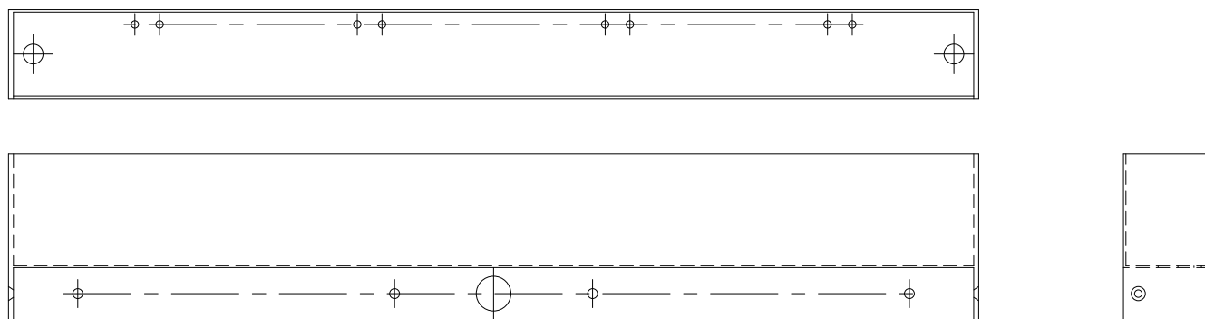
LINEAR LED FIXTURE HOUSING (MXLD-N-S-18-W-24)
