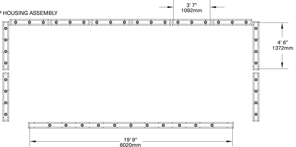
LINEAR LAMP HOUSING
